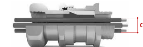
Conduit sealing fitting
